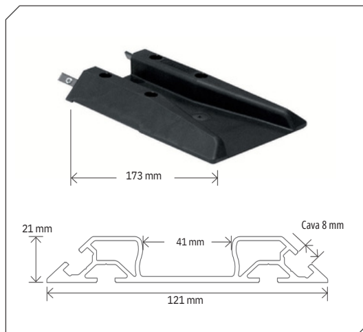
Terminale Fifo Monorail 40 mm
